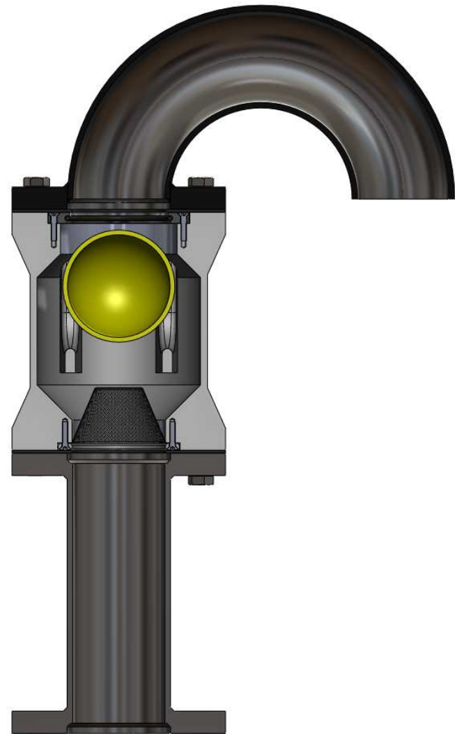
Section View
